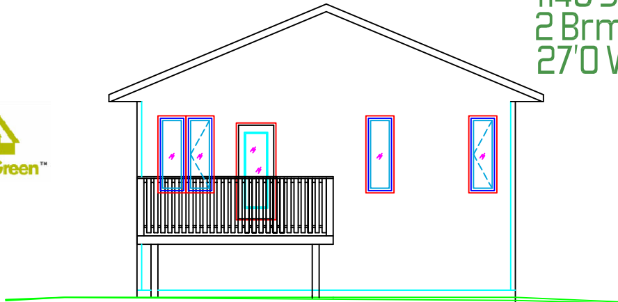
REAR ELEVATION
